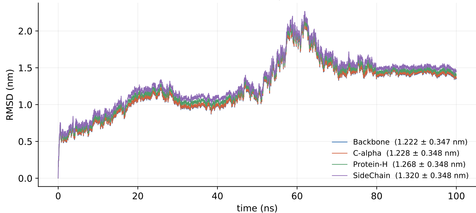
Backbone RMSD from the equilibrated structure
