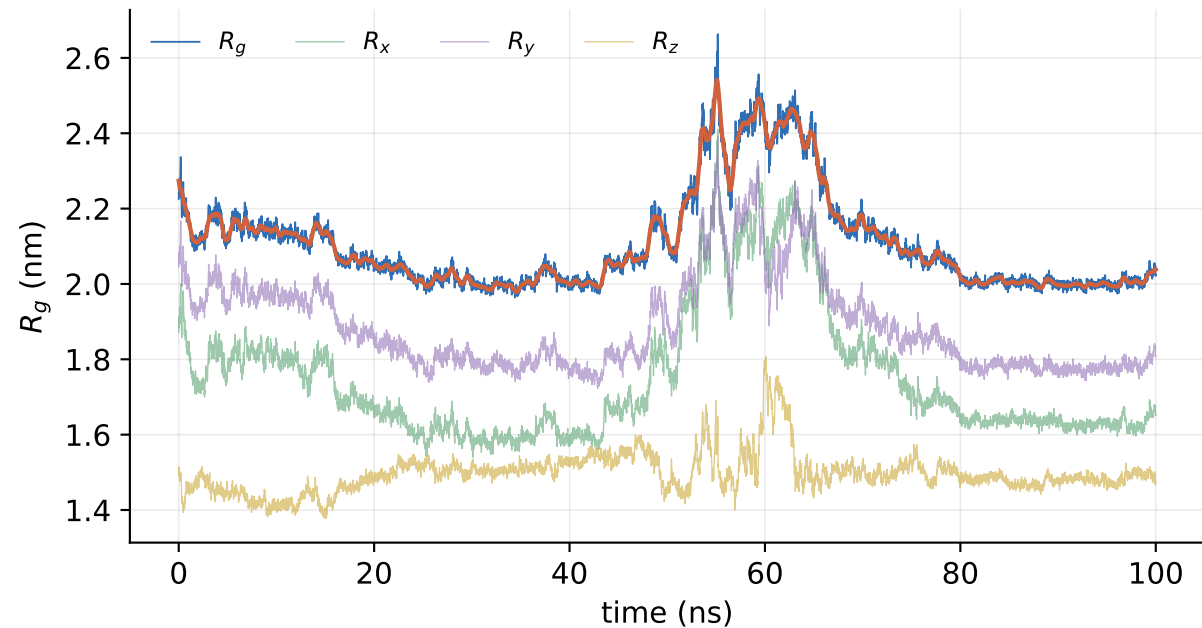
Radius of gyration ( 2.109 \pm 0.132 nm)
