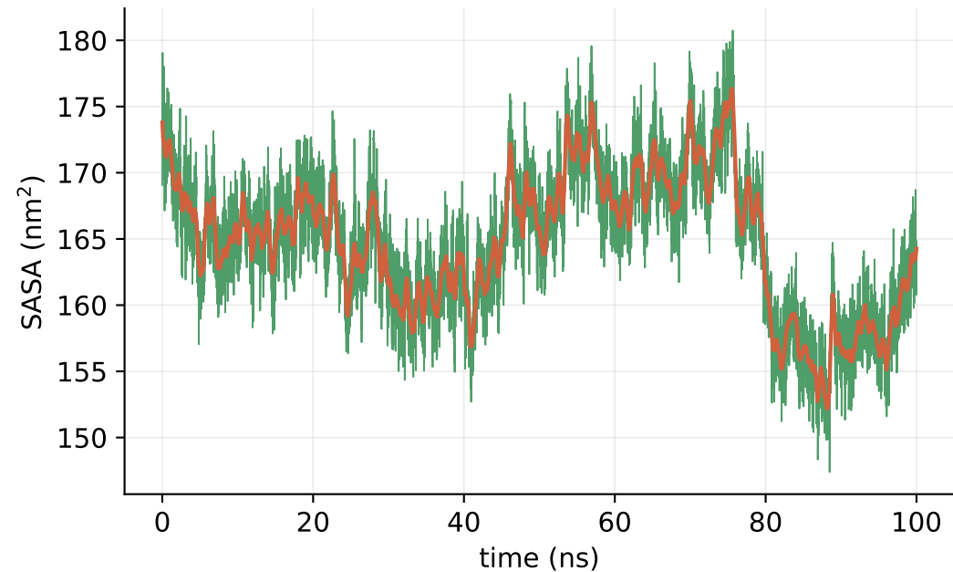
Total solvent-accessible surface ( 164.8 \pm 5.5 \text{ nm}^2 )
