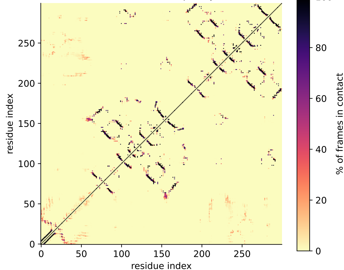
Residue-residue contact frequency ( < 0.45 nm)
