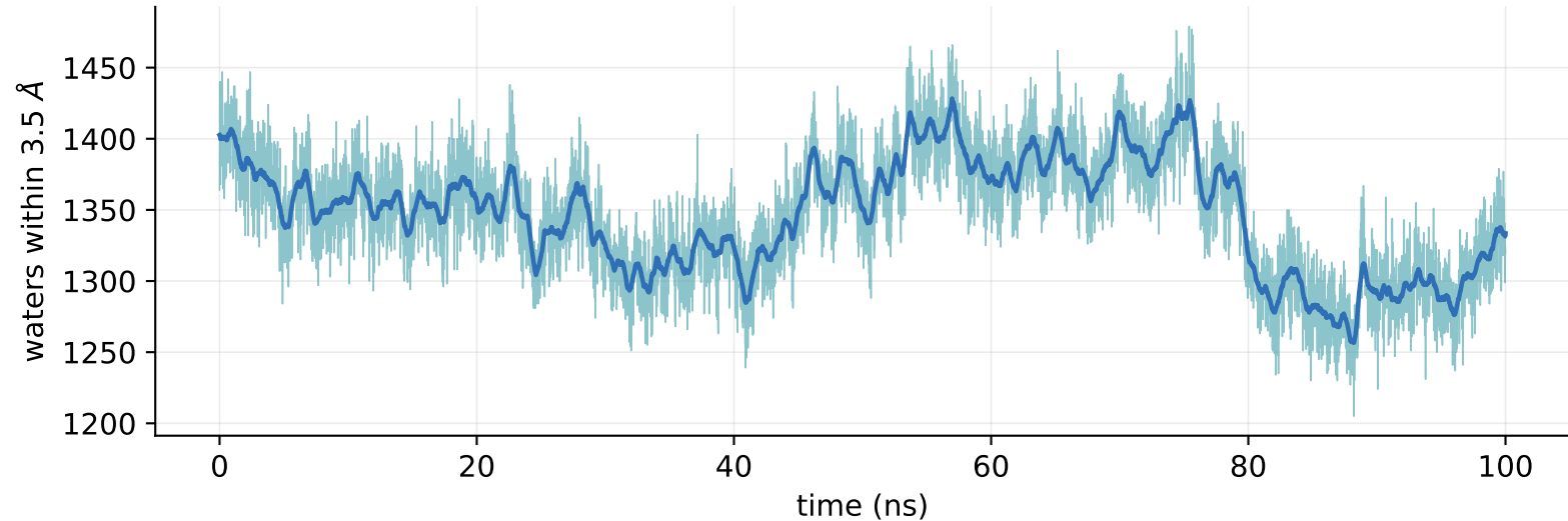
First hydration shell ( 1347 \pm 43 molecules)
