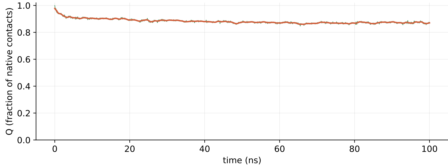
Native-contact retention (final Q = 0.868 )
