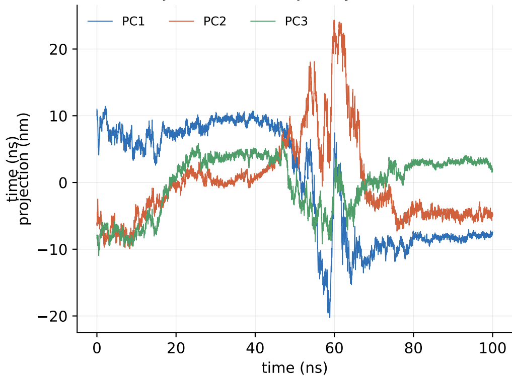
Projection of the trajectory on PC1-PC3
