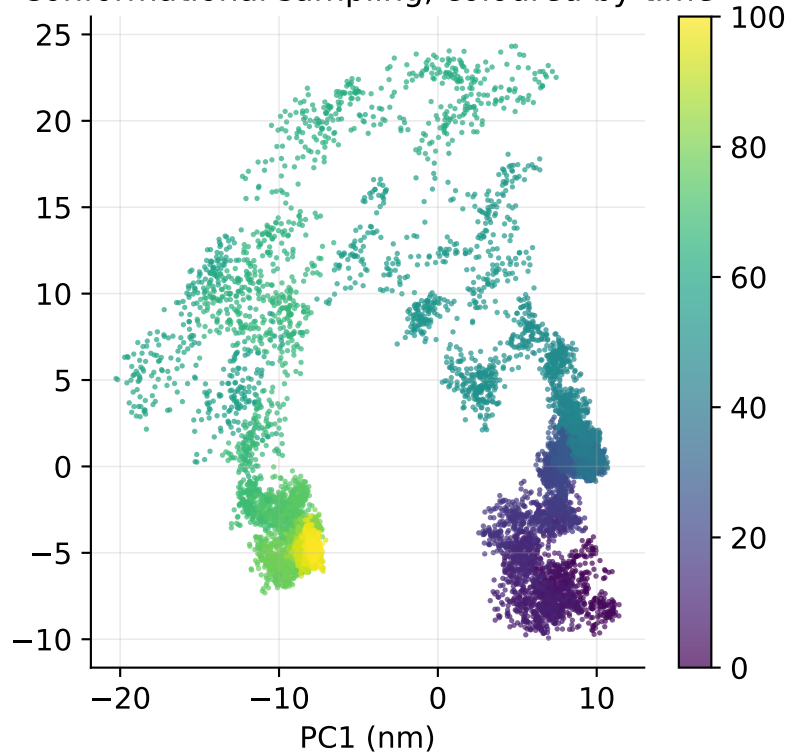
Conformational sampling, coloured by time
