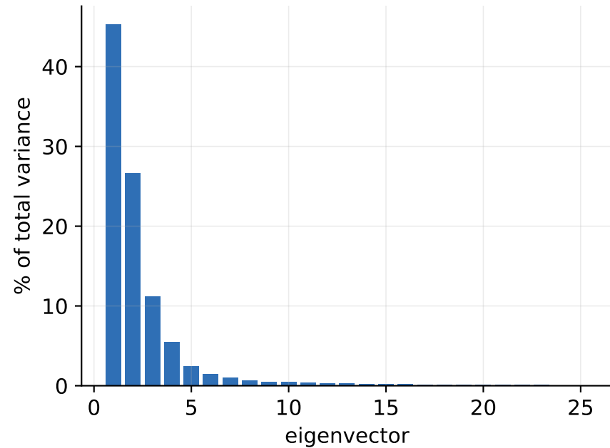
Scree plot
