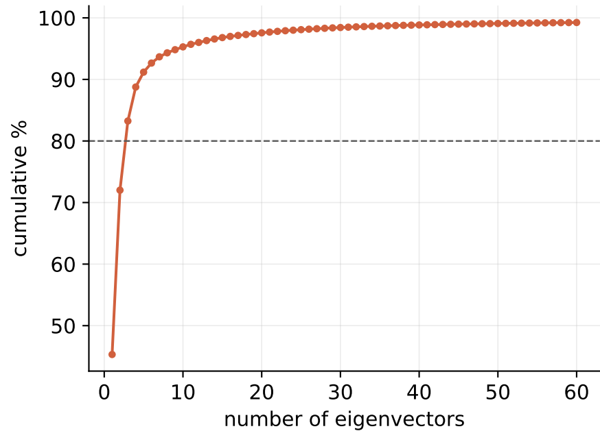
Cumulative variance
